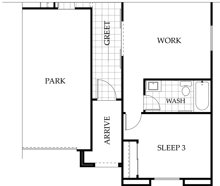
PLAN 7B/7C FIRST FLOOR
